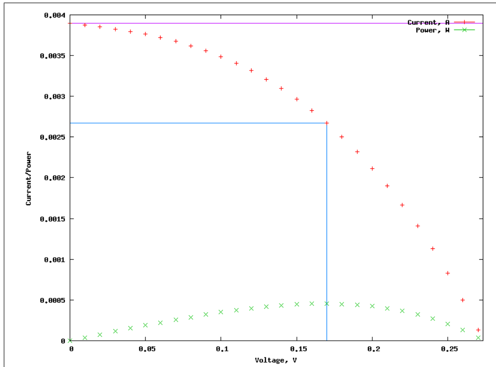
Figure 1: Power (W) and Current (A) versus Voltage (V)
